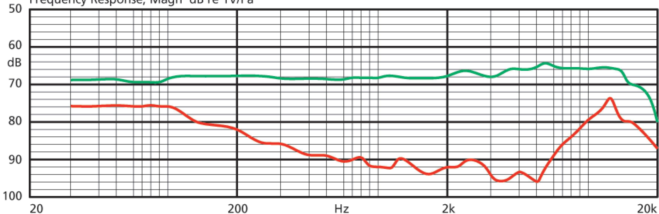
Frequency Response, Magn dB re 1V/Pa
