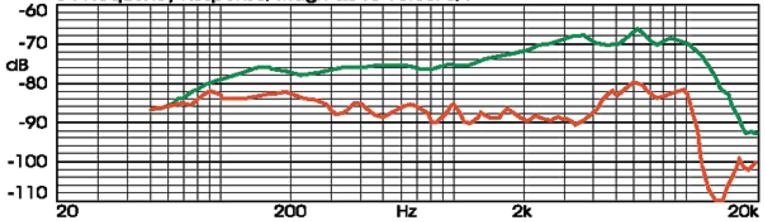
B : Frequency Response, Magn db re 10.00Pa/V
