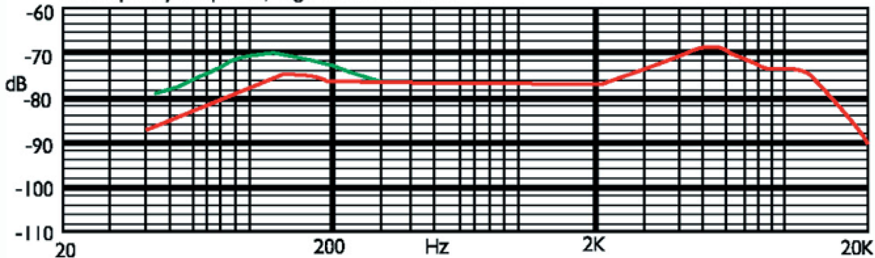
A: Frequency Response, Magn dB re 10.00V/Pa
