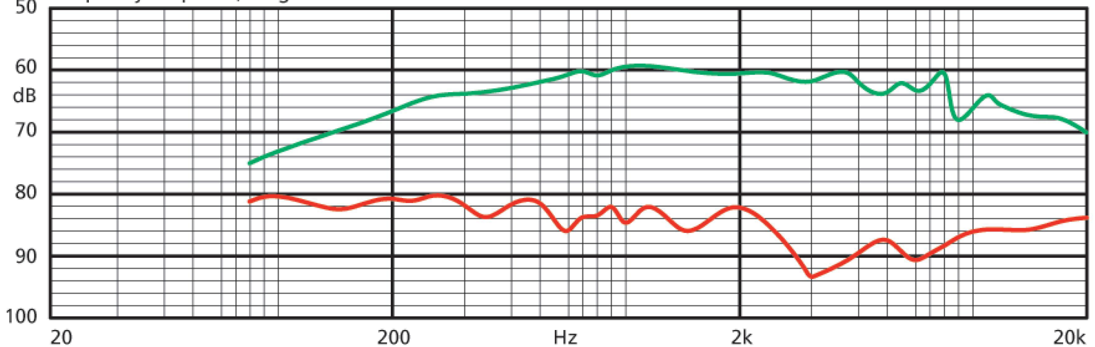
Frequency Response, Magn dB re 1V/Pa
